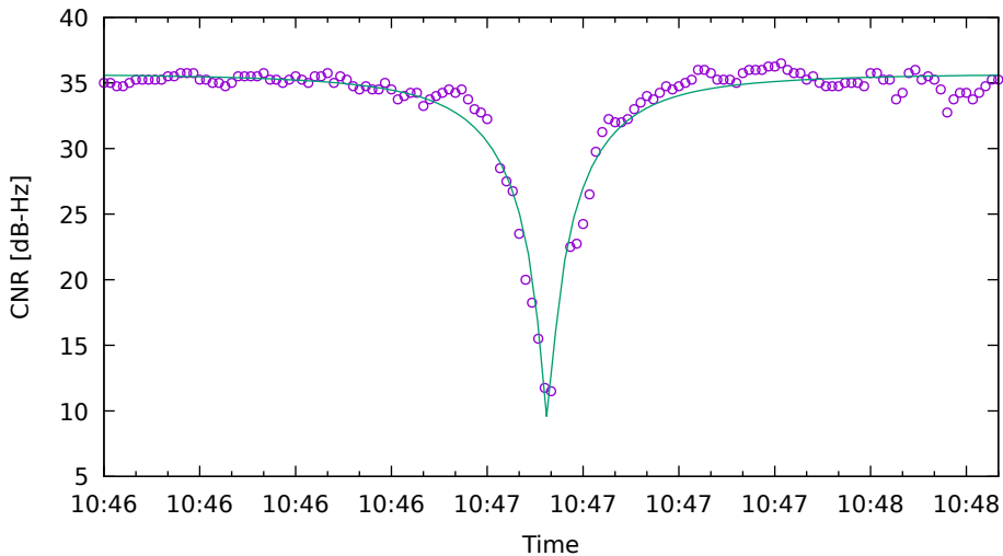
CNR fit for R01 on XiaomiMi8 - drive 3 (DOY262)
