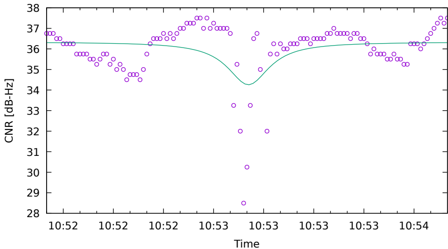
CNR fit for R01 on XiaomiMi8 - drive 6 (DOY262)
