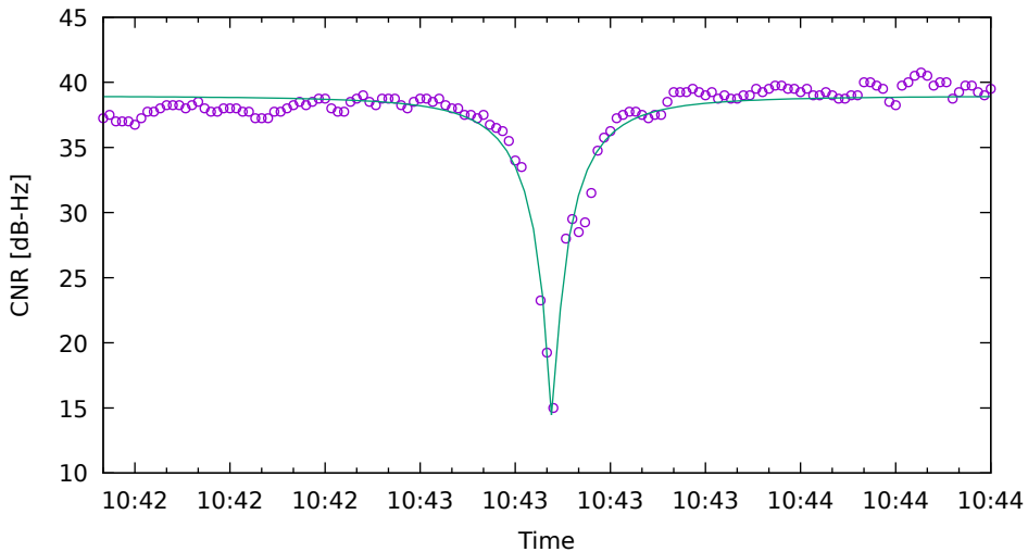
CNR fit for R08 on XiaomiMi8 - drive 1 (DOY262)
