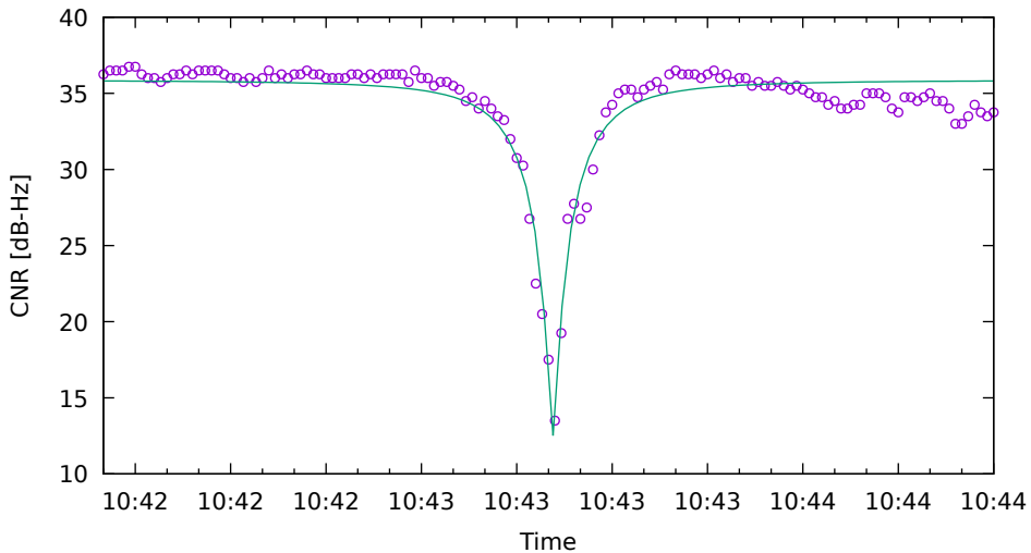
CNR fit for R23 on XiaomiMi8 - drive 1 (DOY262)
