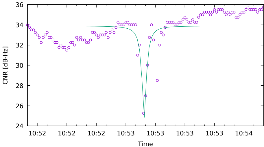
CNR fit for R23 on XiaomiMi8 - drive 6 (DOY262)
