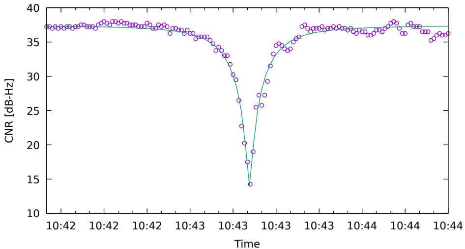
CNR fit for R24 on XiaomiMi8 - drive 1 (DOY262)
