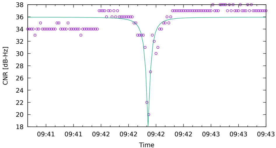
CNR fit for C05 on HuaweiP40 - drive 2 (DOY263)
