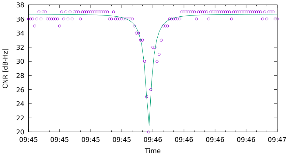
CNR fit for C05 on HuaweiP40 - drive 4 (DOY263)
