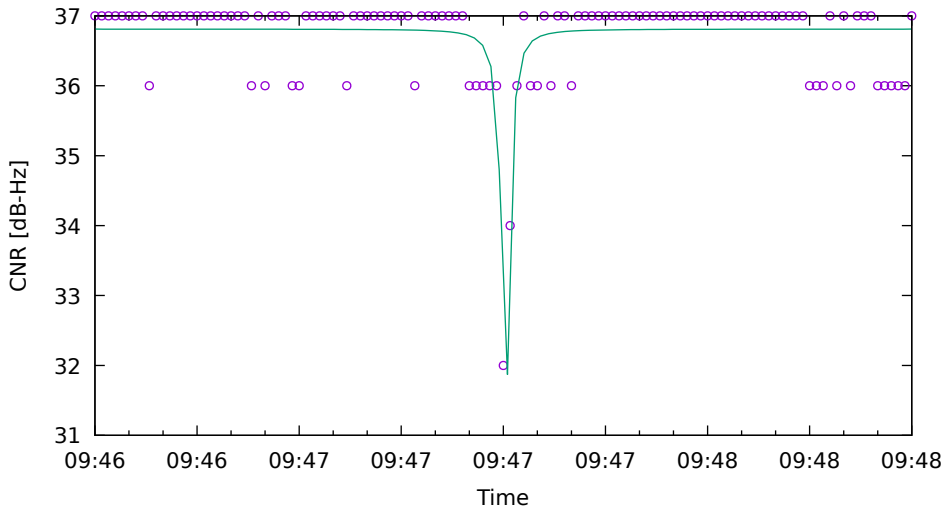
CNR fit for C05 on HuaweiP40 - drive 5 (DOY263)
