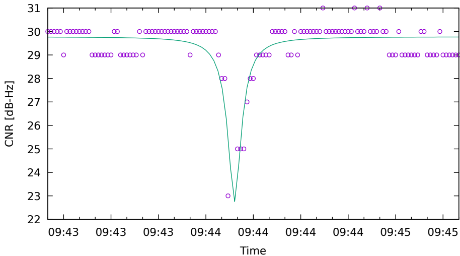
CNR fit for C06 on HuaweiP40 - drive 3 (DOY263)
