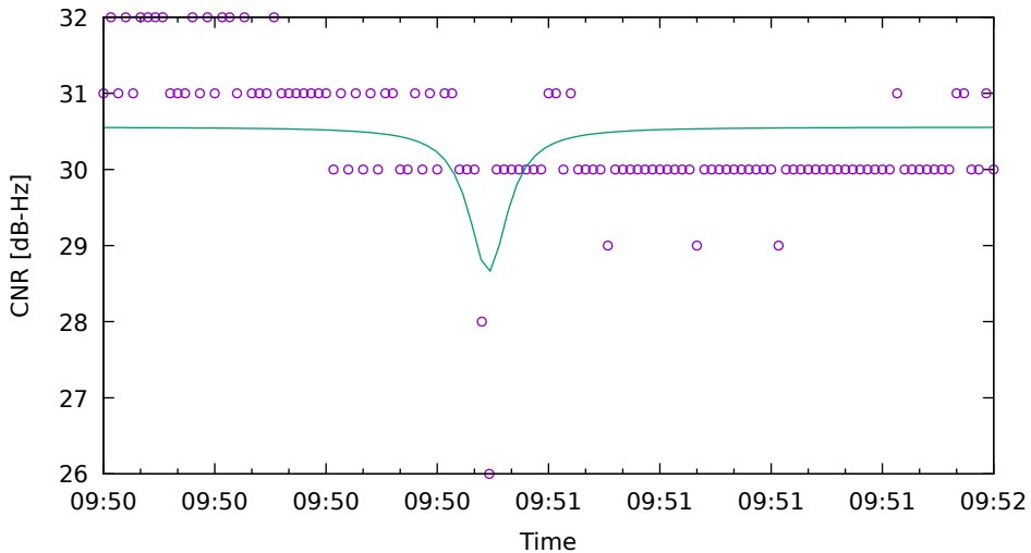
CNR fit for C06 on HuaweiP40 - drive 7 (DOY263)
