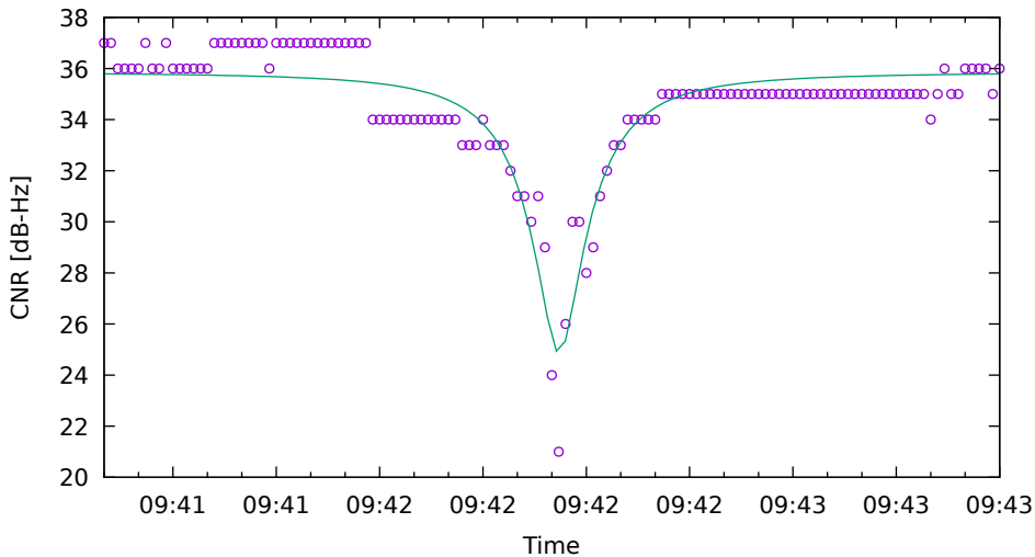
CNR fit for C09 on HuaweiP40 - drive 2 (DOY263)
