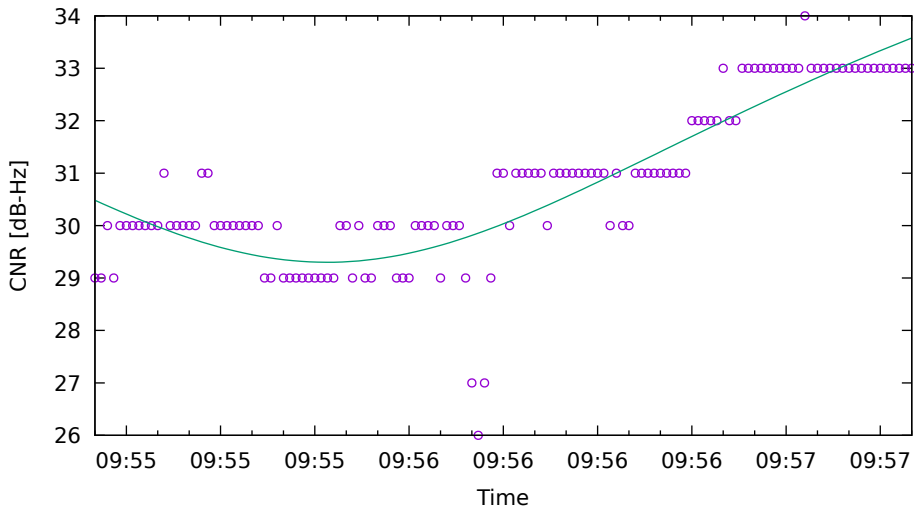
CNR fit for C11 on HuaweiP40 - drive 10 (DOY263)
