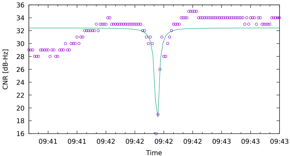
CNR fit for C11 on HuaweiP40 - drive 2 (DOY263)
