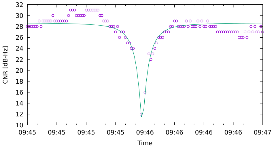
CNR fit for C11 on HuaweiP40 - drive 4 (DOY263)
