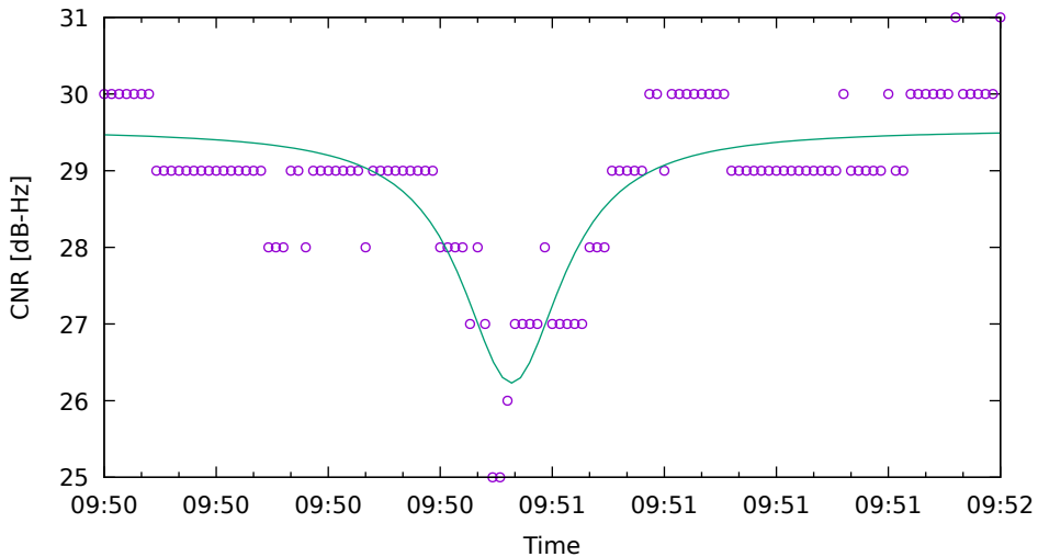
CNR fit for C11 on HuaweiP40 - drive 7 (DOY263)
