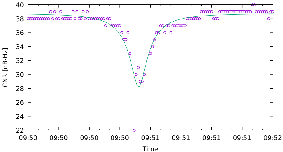
CNR fit for G03 on HuaweiP40 - drive 7 (DOY263)
