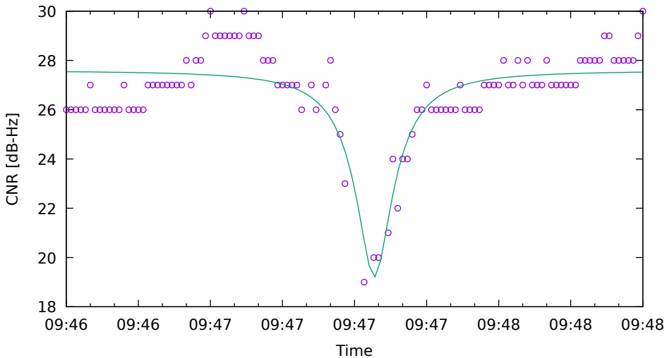
CNR fit for G08 on HuaweiP40 - drive 5 (DOY263)
