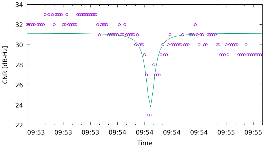
CNR fit for G08 on HuaweiP40 - drive 9 (DOY263)
