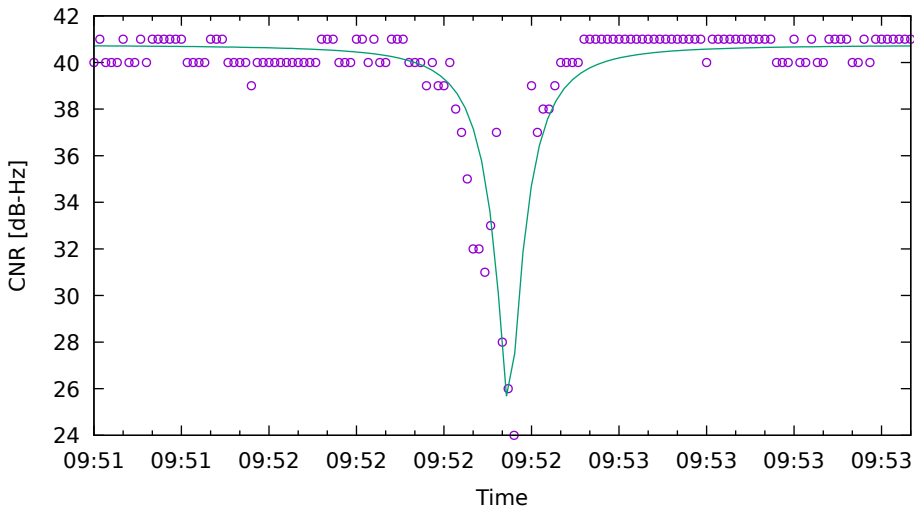
CNR fit for G17 on HuaweiP40 - drive 8 (DOY263)
