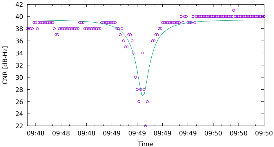
CNR fit for G32 on HuaweiP40 - drive 6 (DOY263)
