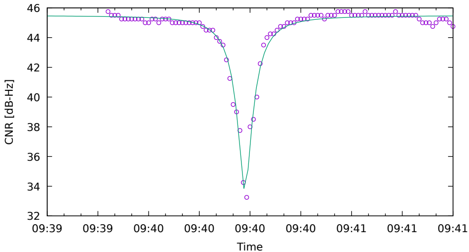
CNR fit for C05 on SamsungS20 - drive 1 (DOY263)
