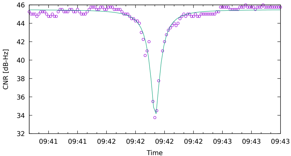
CNR fit for C05 on SamsungS20 - drive 2 (DOY263)
