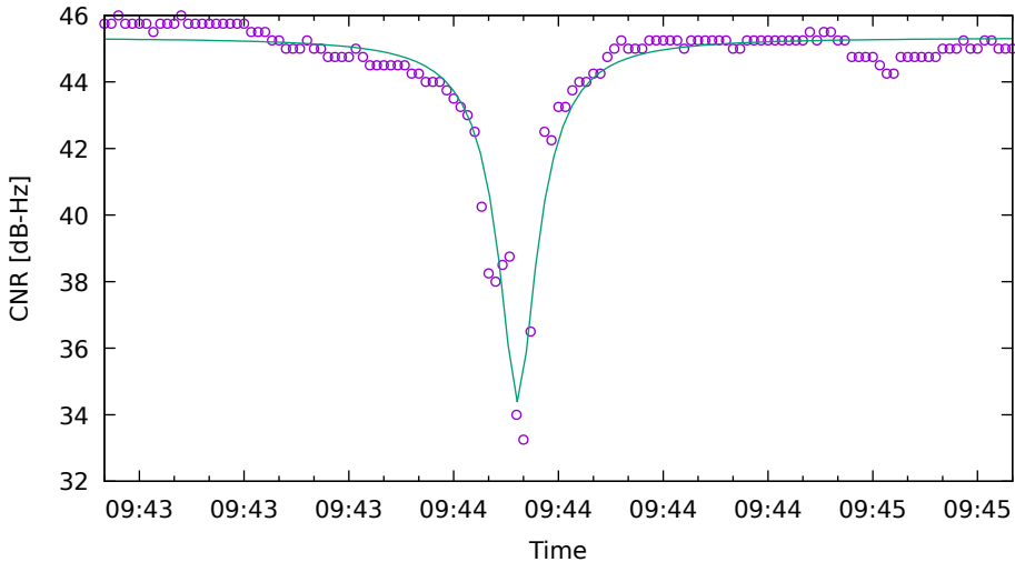
CNR fit for C05 on SamsungS20 - drive 3 (DOY263)
