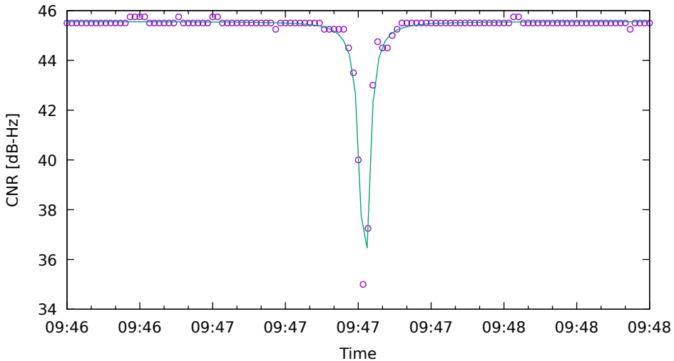
CNR fit for C05 on SamsungS20 - drive 5 (DOY263)
