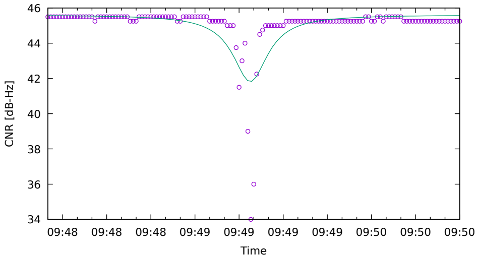
CNR fit for C05 on SamsungS20 - drive 6 (DOY263)
