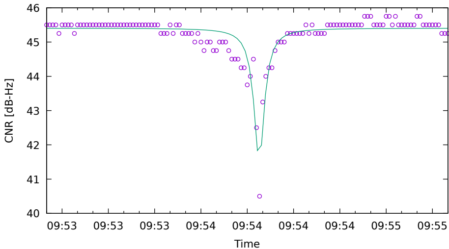
CNR fit for C05 on SamsungS20 - drive 9 (DOY263)
