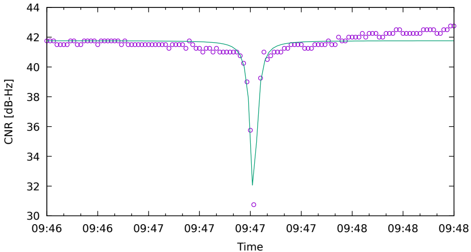
CNR fit for C16 on SamsungS20 - drive 5 (DOY263)
