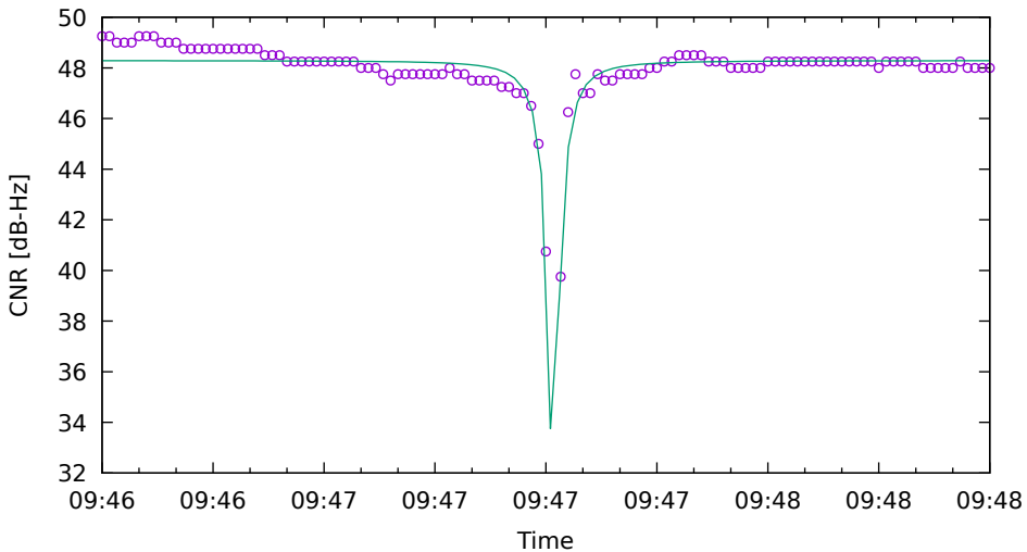
CNR fit for C34 on SamsungS20 - drive 5 (DOY263)
