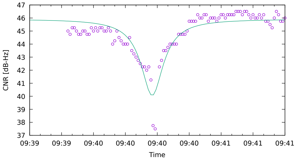
CNR fit for E04 on SamsungS20 - drive 1 (DOY263)
