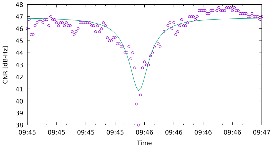
CNR fit for E04 on SamsungS20 - drive 4 (DOY263)
