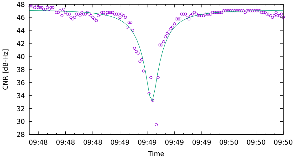
CNR fit for E04 on SamsungS20 - drive 6 (DOY263)
