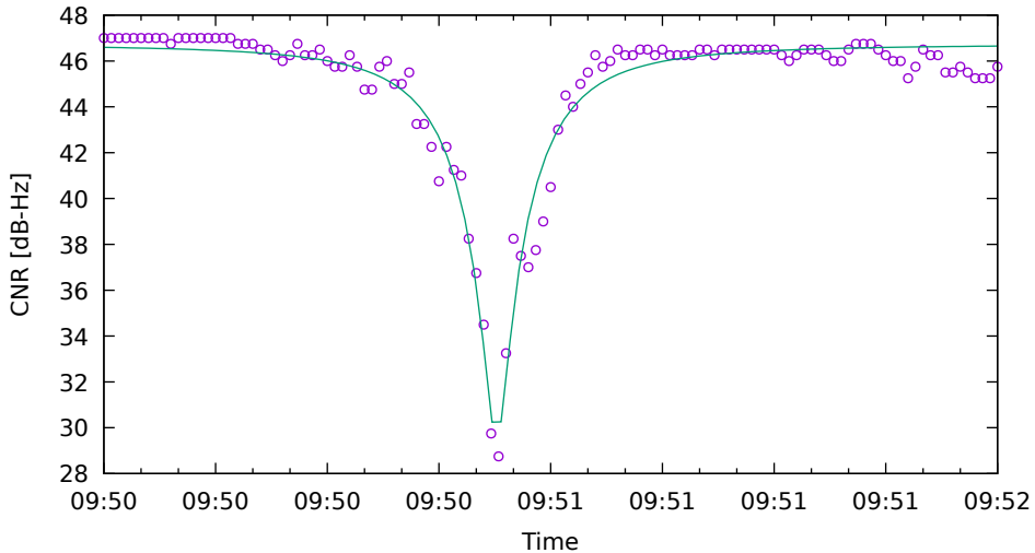
CNR fit for E04 on SamsungS20 - drive 7 (DOY263)
