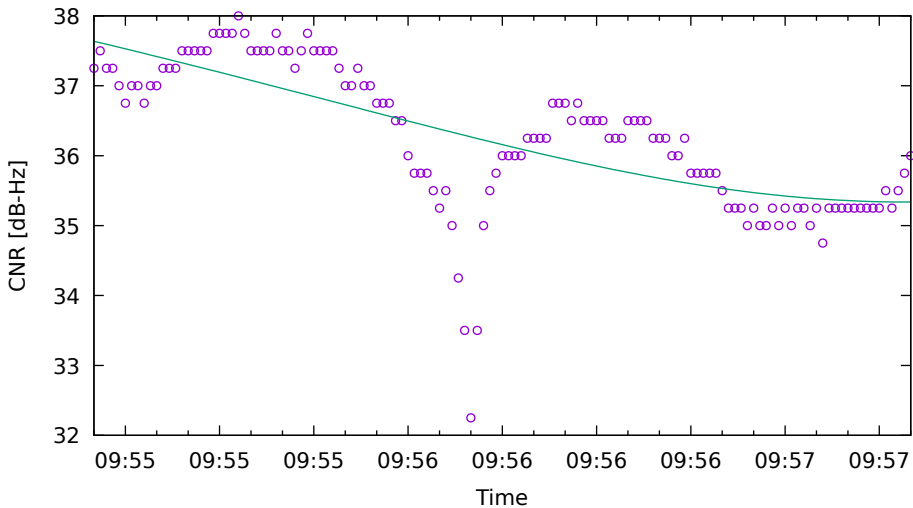
CNR fit for E12 on SamsungS20 - drive 10 (DOY263)
