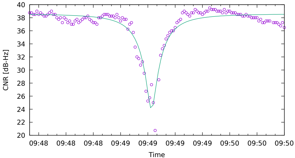
CNR fit for E12 on SamsungS20 - drive 6 (DOY263)
