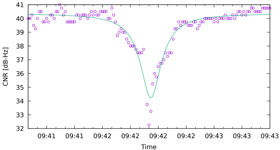
CNR fit for E19 on SamsungS20 - drive 2 (DOY263)
