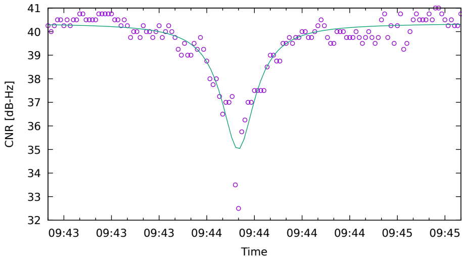
CNR fit for E19 on SamsungS20 - drive 3 (DOY263)
