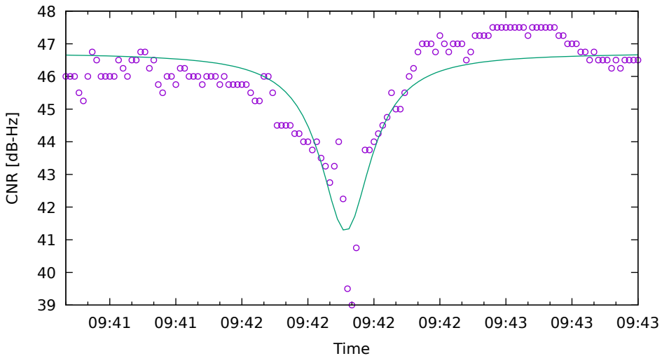
CNR fit for E33 on SamsungS20 - drive 2 (DOY263)
