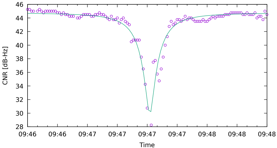
CNR fit for E33 on SamsungS20 - drive 5 (DOY263)
