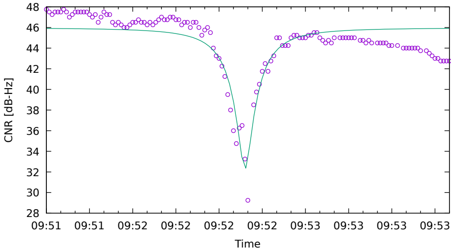
CNR fit for E33 on SamsungS20 - drive 8 (DOY263)
