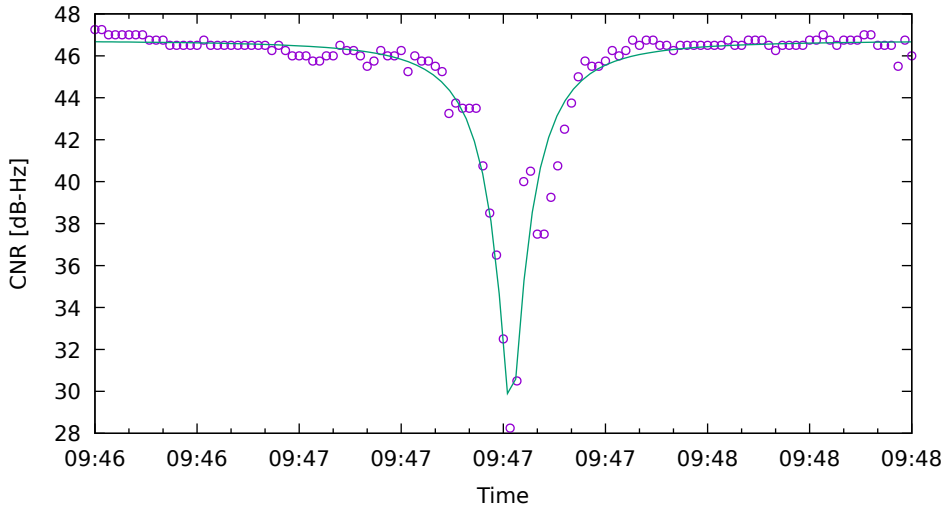
CNR fit for G01 on SamsungS20 - drive 5 (DOY263)
