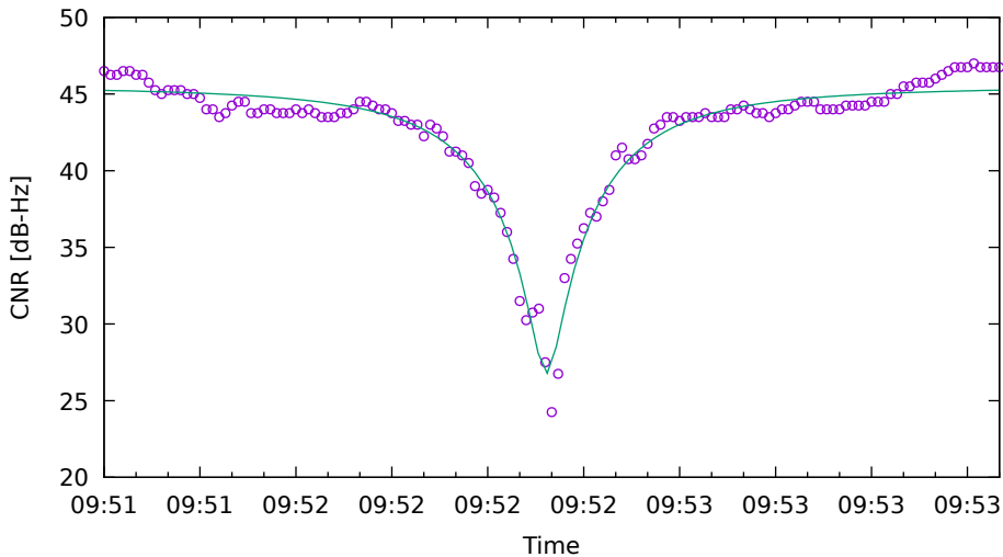
CNR fit for G01 on SamsungS20 - drive 8 (DOY263)
