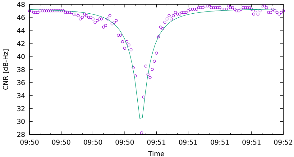
CNR fit for G03 on SamsungS20 - drive 7 (DOY263)
