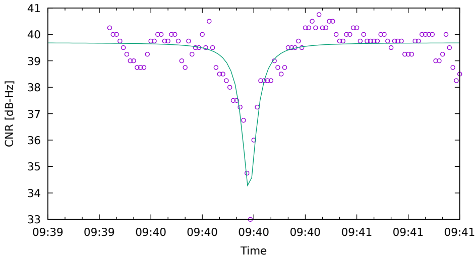
CNR fit for G08 on SamsungS20 - drive 1 (DOY263)
