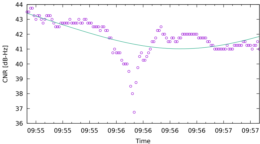
CNR fit for G08 on SamsungS20 - drive 10 (DOY263)
