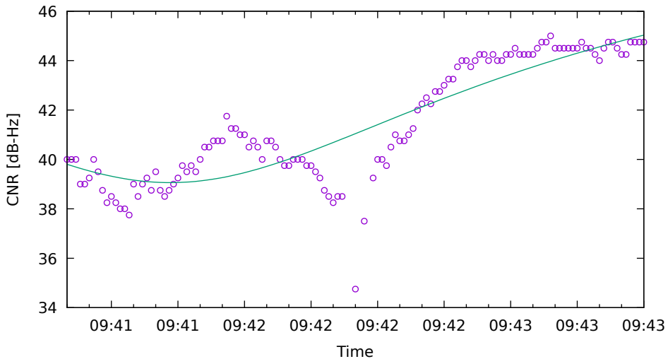
CNR fit for G08 on SamsungS20 - drive 2 (DOY263)
