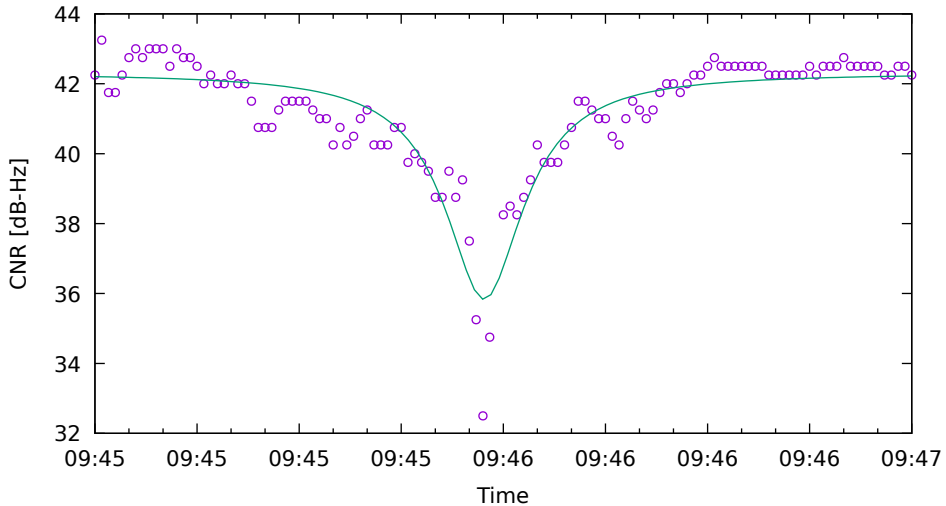
CNR fit for G08 on SamsungS20 - drive 4 (DOY263)
