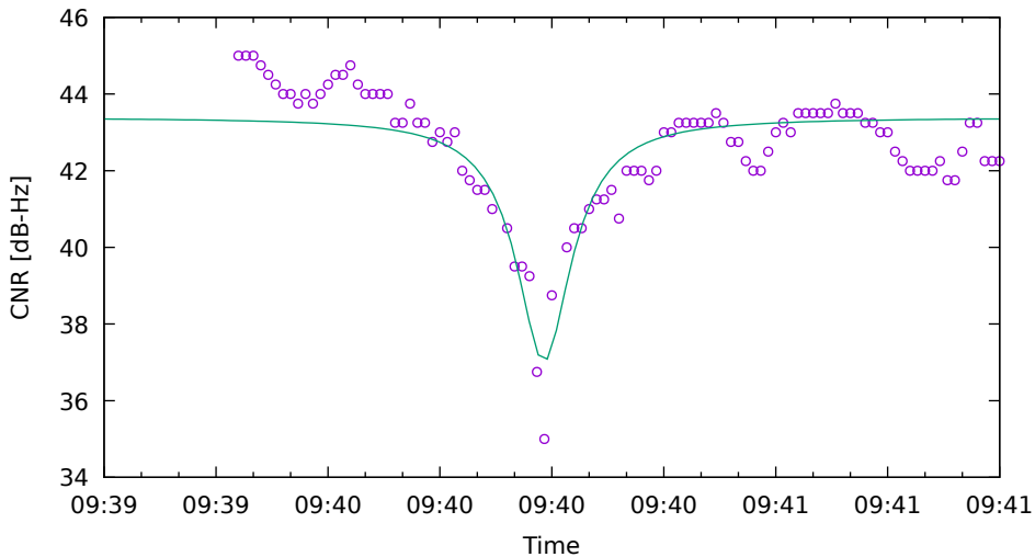
CNR fit for G32 on SamsungS20 - drive 1 (DOY263)
