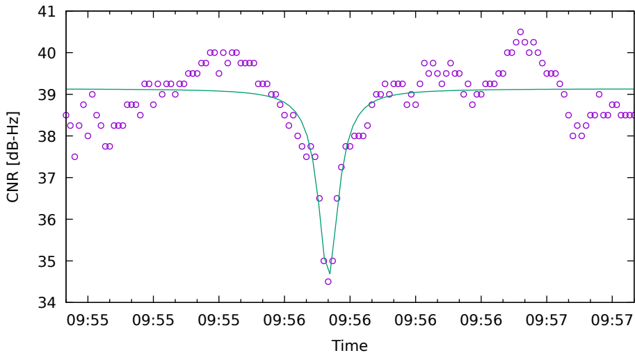
CNR fit for G32 on SamsungS20 - drive 10 (DOY263)
