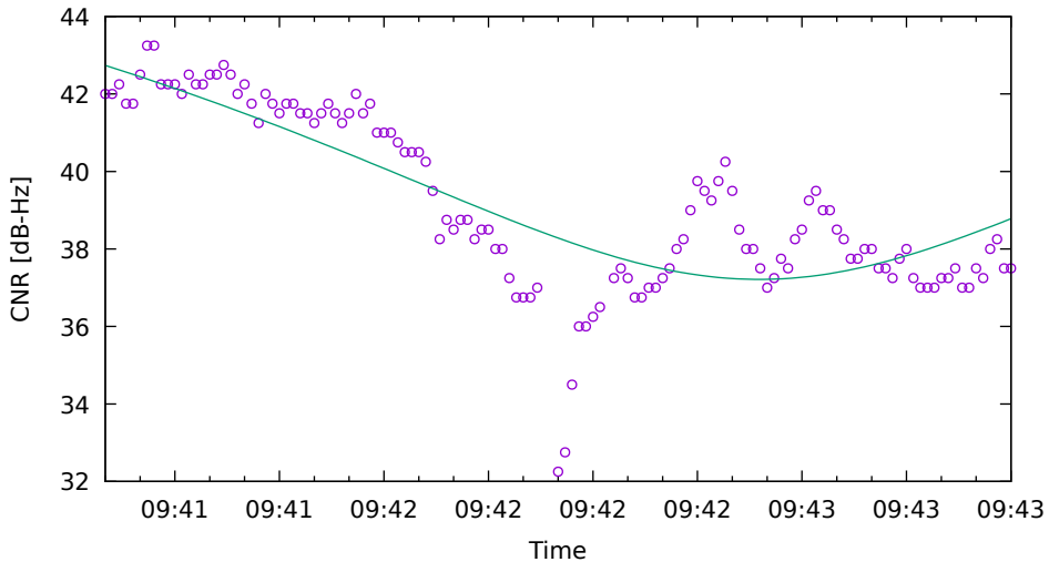
CNR fit for G32 on SamsungS20 - drive 2 (DOY263)
